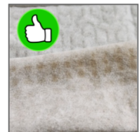
Good Sampling
